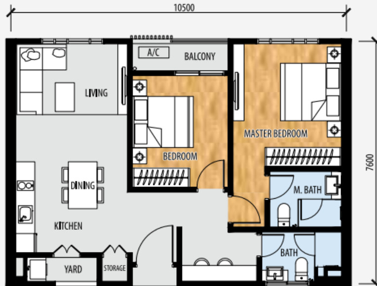
Type B1 2 Bedrooms, 2 Baths 858 sq ft • 79.70 sqm
