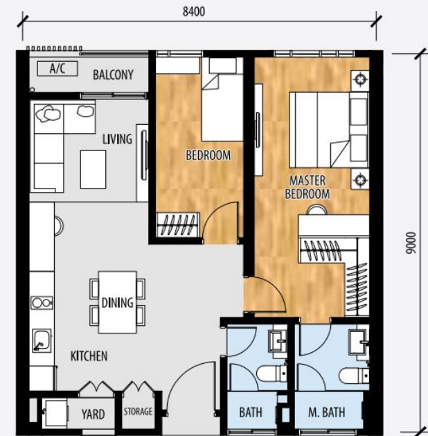
Type B2 2 Bedrooms, 2 Baths 812 sq ft • 75.45 sqm
