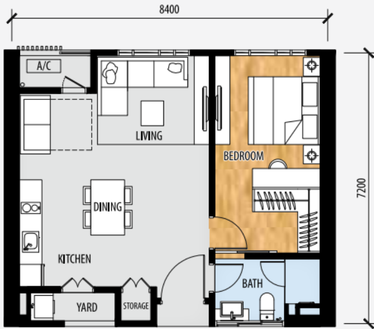
Type A 1 Bedroom, 1 Bath 650 sq ft • 60.40 sqm
